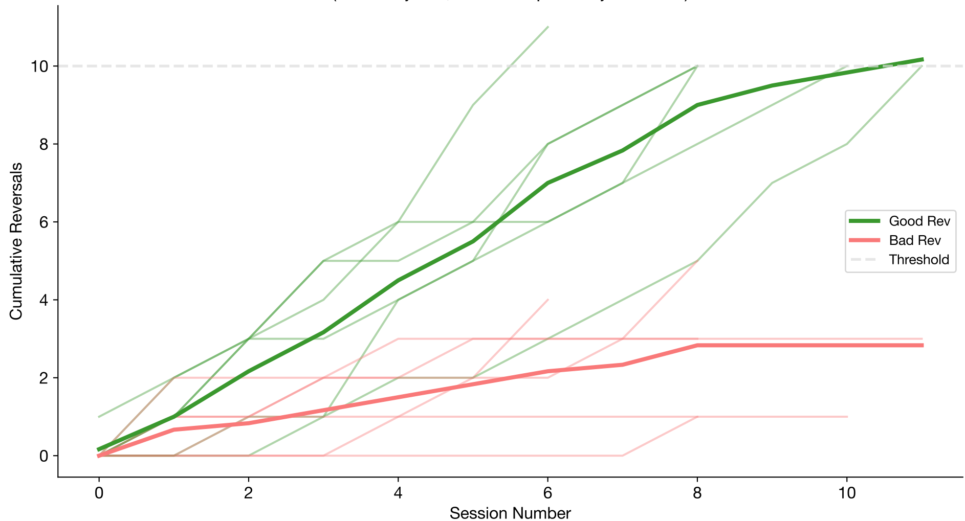
Cumulative Good and Bad Reversals Over Time (n=6 subjects; sessions per subject=7-12)
